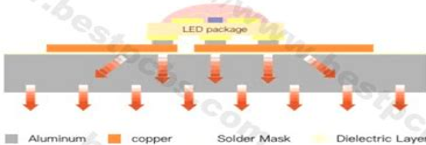
aluminum LED PCB structure
