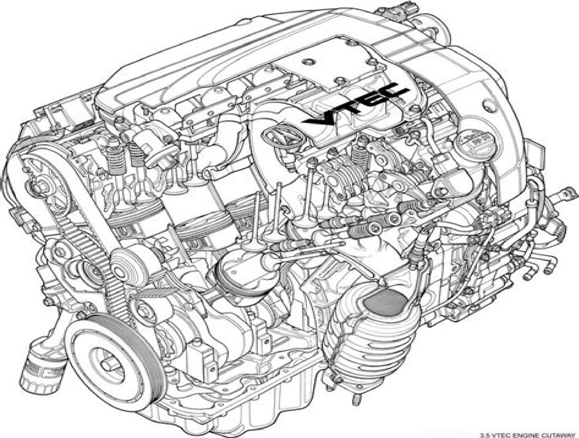
3.5 VTEC ENGINE CUTAWAY
