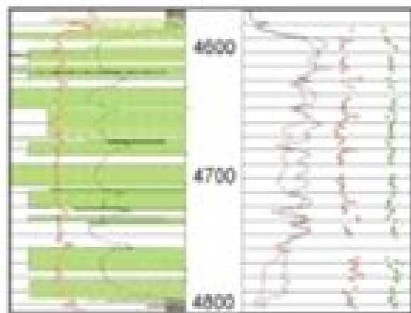
Conventional logs
