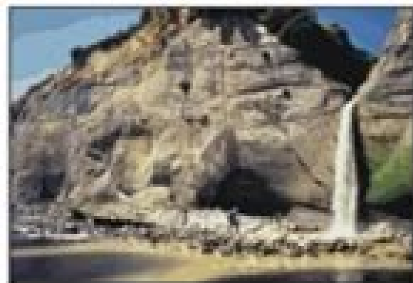
Outcrops
