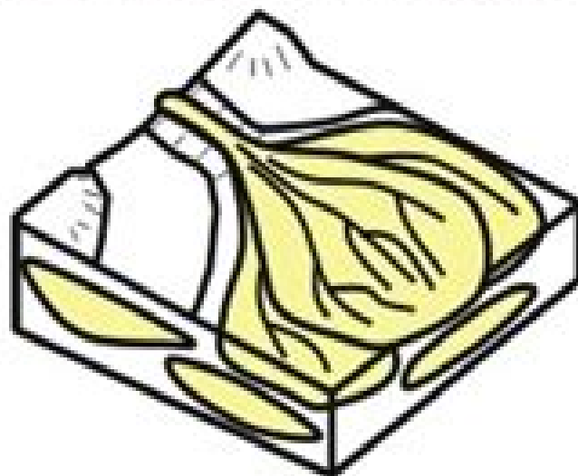
Conceptual model
