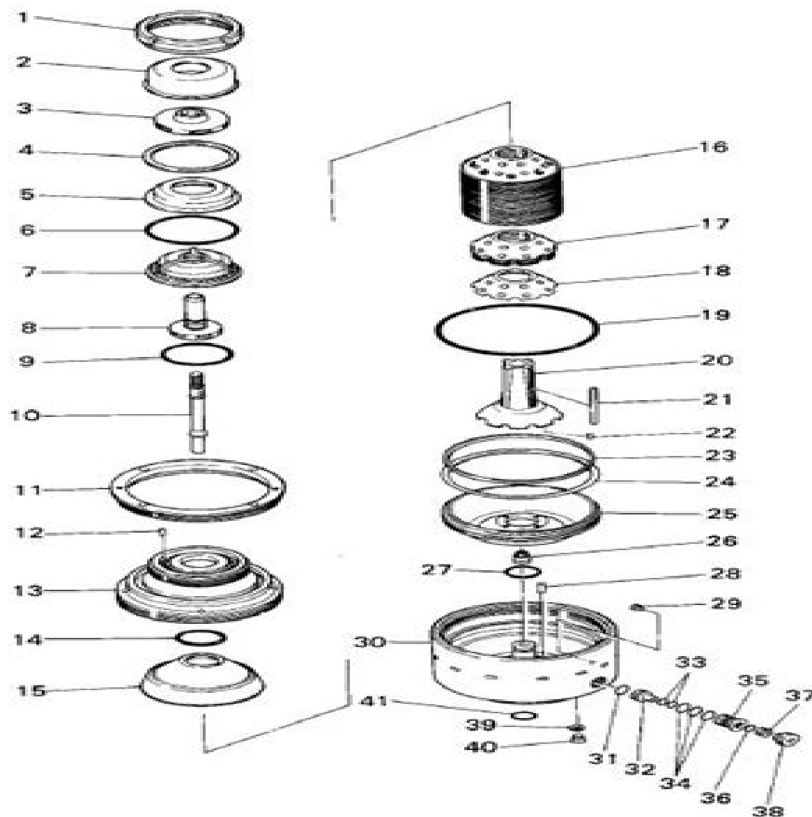
Fig. 6-24 Illustration of bowl parts
