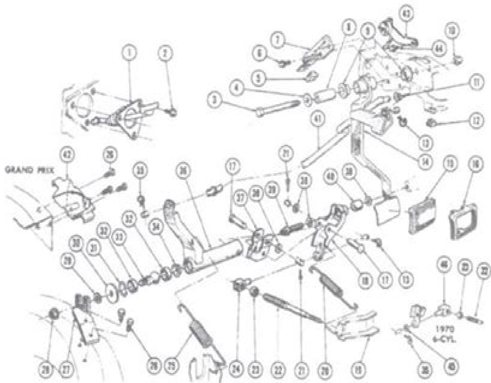
1960-72 CLUTCH LINKAGE
