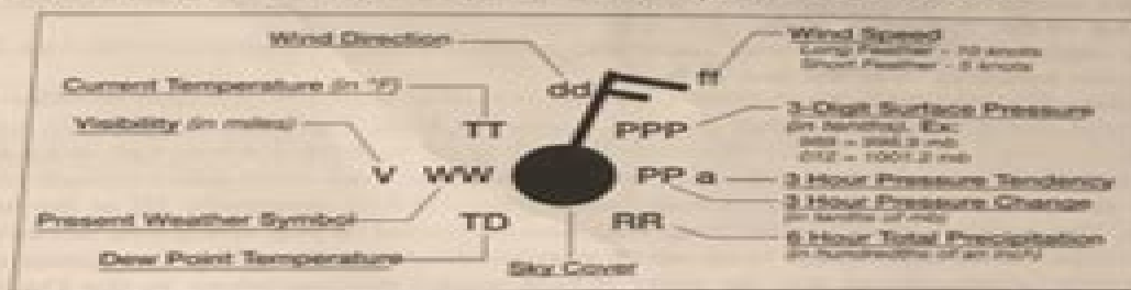
Figure 19-1: Sample weather station model. (Adapted from National Weather Service)
