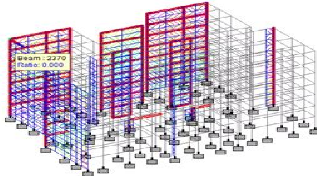
figure 4.4.3.3b Wind Load
