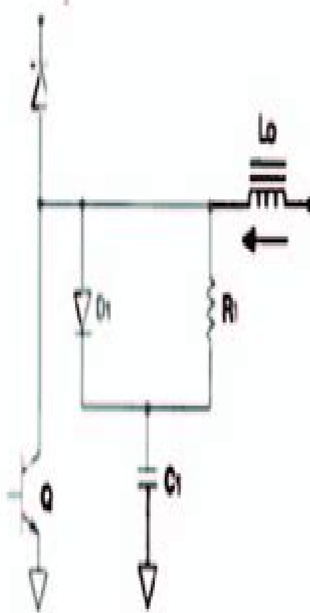
Fig 2b. RCD Snubber circuit
