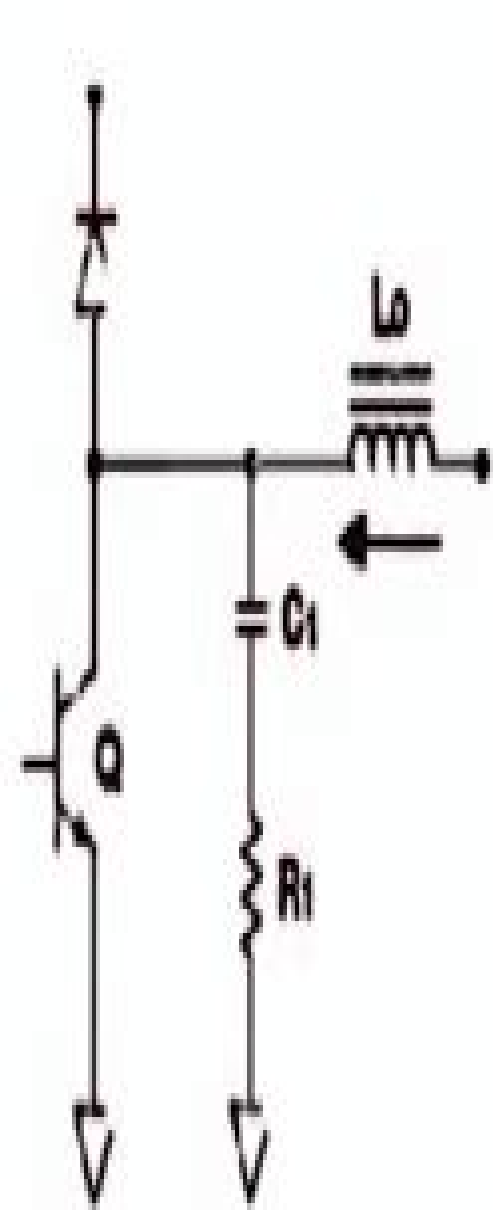
Fig 2a. RC Snubber circuit
