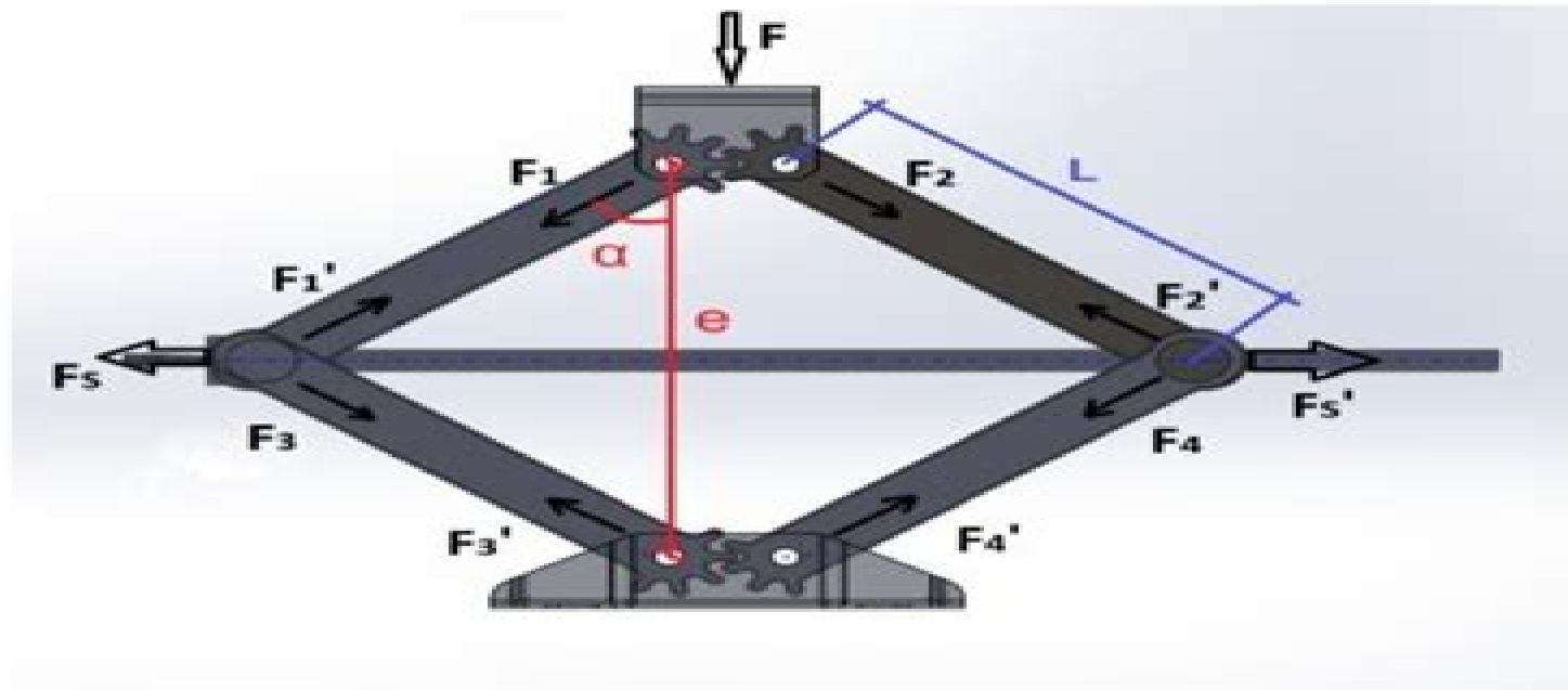
Figure 3: Forces in Scissor Jack members
