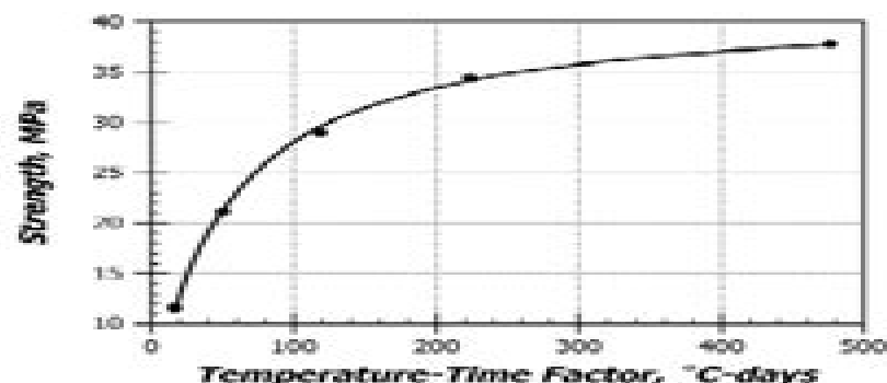
FIG. 1 Example of a Relationship Between Compressive Strength and Temperature-Time Factor
