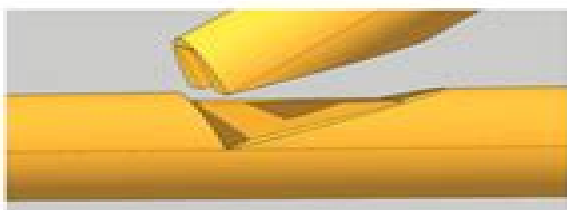
Figure 25: The hinge point is half way through the log. If we removed all that wood from the tie beam, it would be much too weak. So we leave a large block of wood — a tenon—in the beam.
