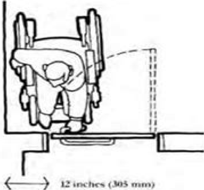
C. Minimum Clearance
