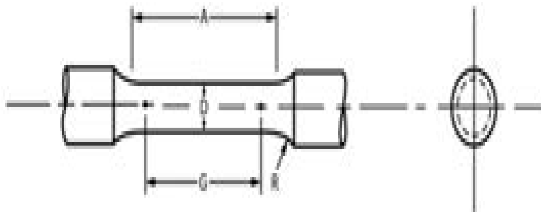
Dimensions, mm [in.] For Test Specimens with Gauge Length Four Times the Diameter [E8]
