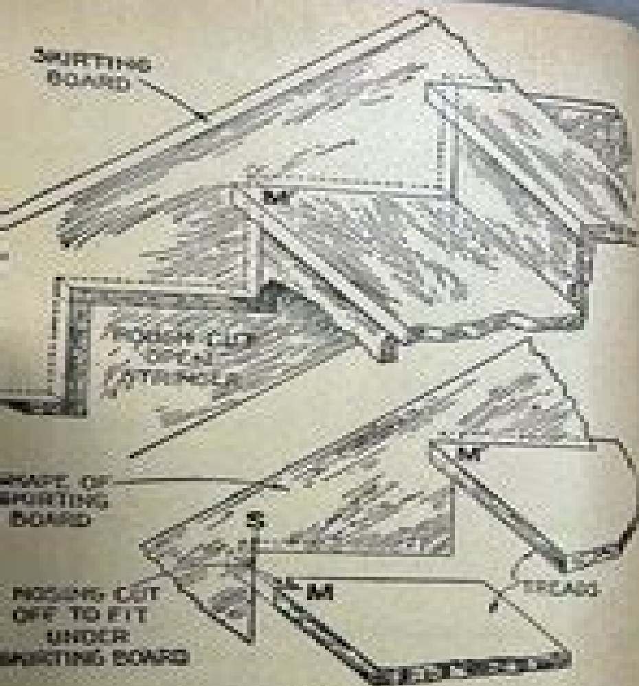
Detail of Stair Construction
