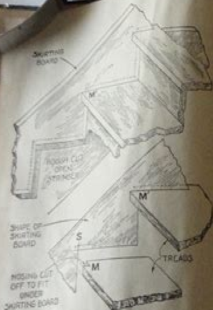
Detail of Stair Construction
