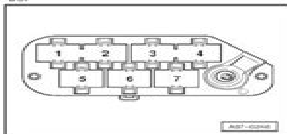
Connector station E-box, plenum chamber
