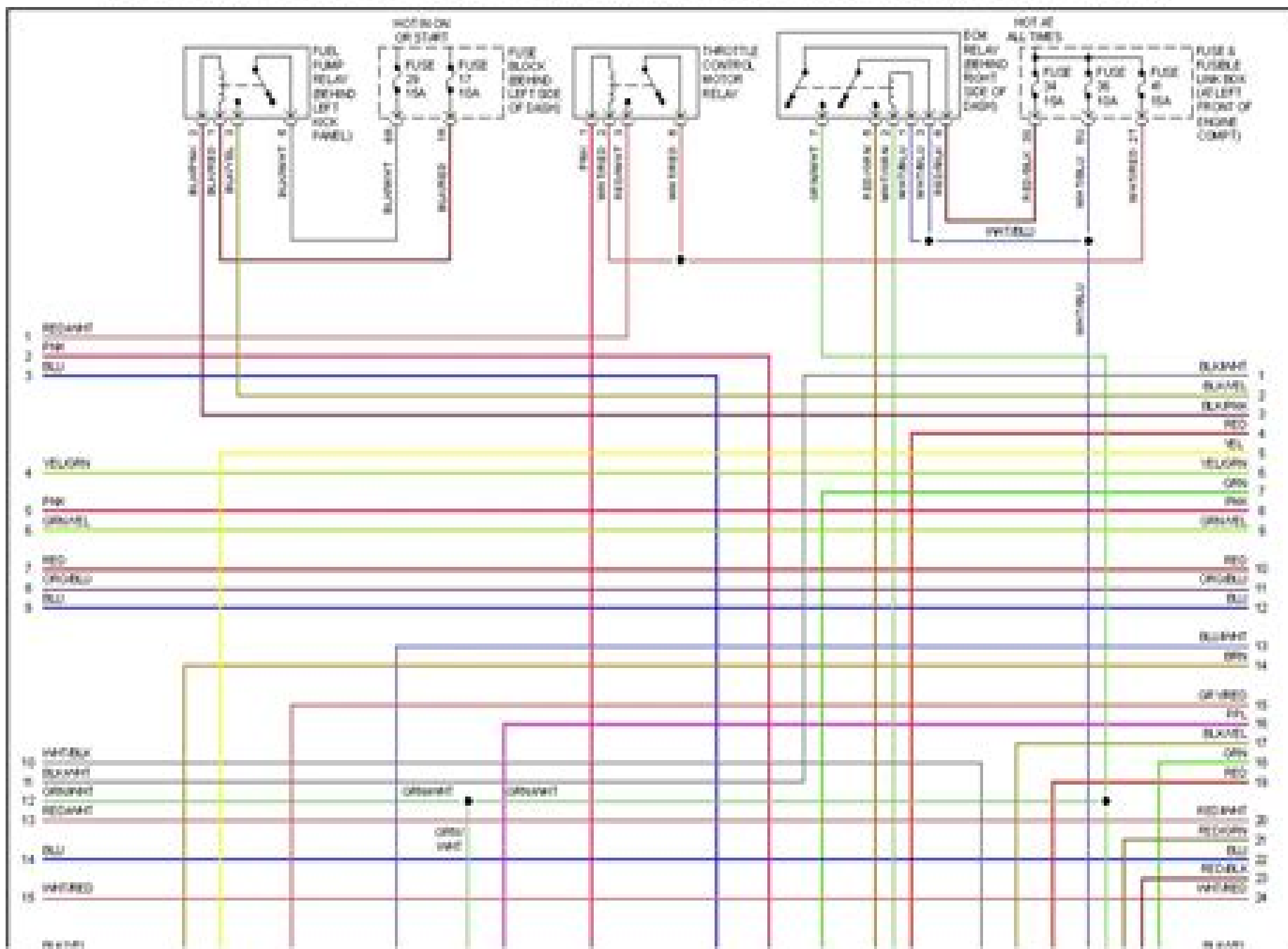
2003 Nissan Sentra GXE-Fig. 17: 1.8L, Engine Performance Circuit, SULEV (2 of 4)
