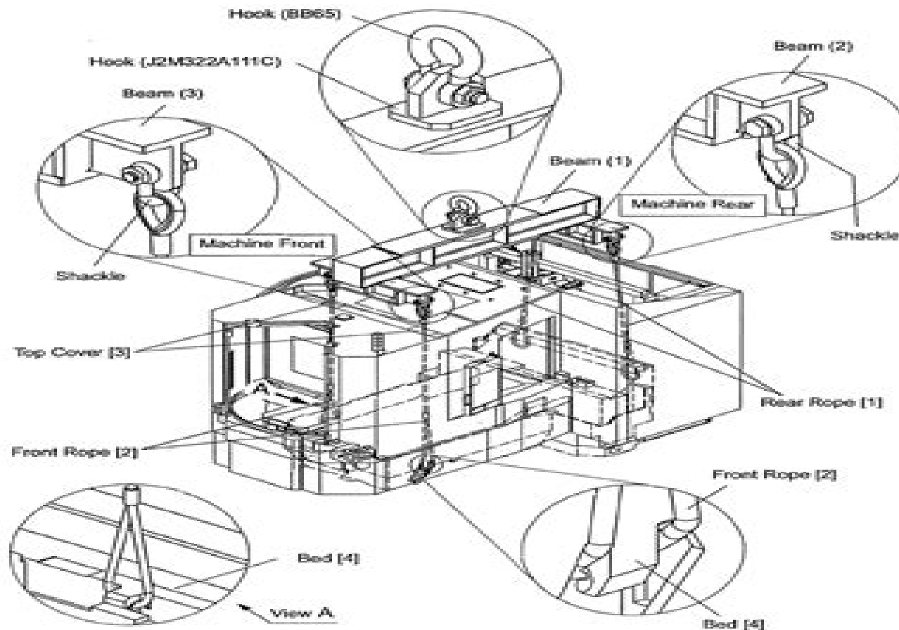
Figure 3.1 Lifting Main Machine (Using 4-Point Lifting Equipment: a81/a82)
