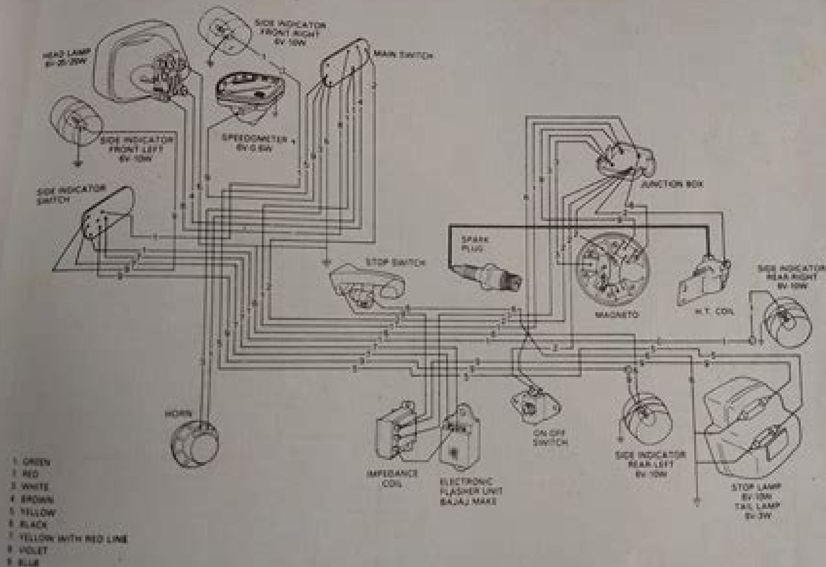
Fig. 21 (c) Wiring diagram for bajaj-Super with A. C. Blinkers ('bajaj' make)
