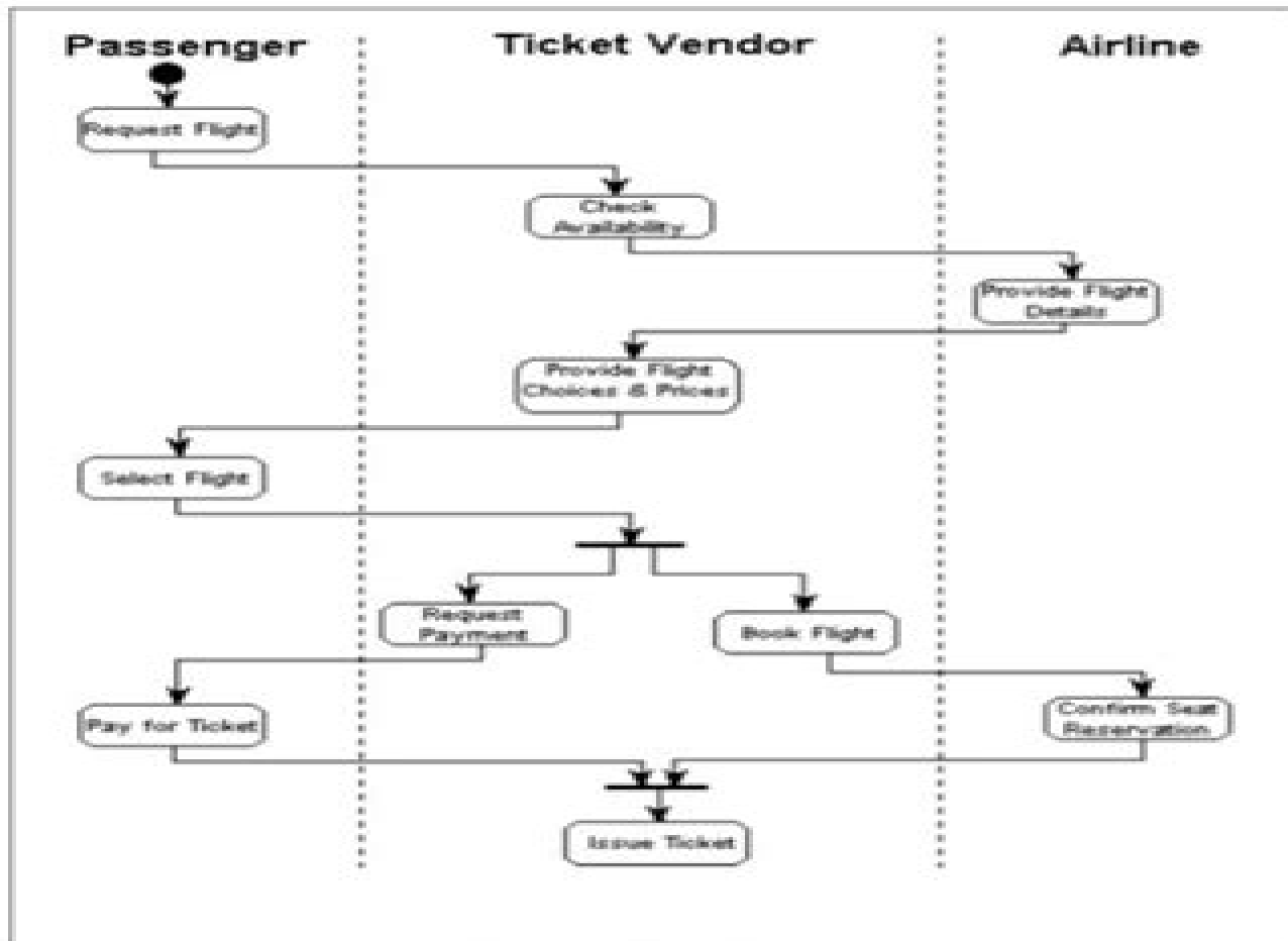
Figure 2 Activity Diagram
