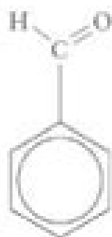
8 Benzaldehyde, \text{C}_6\text{H}_5\text{CHO}
