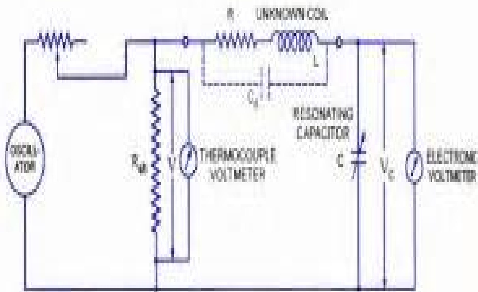
Circuit Diagram of a Q-meter
