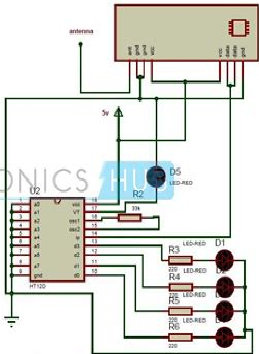
RF receiver
