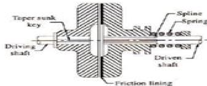
Fig 1.1 Single plate clutch
