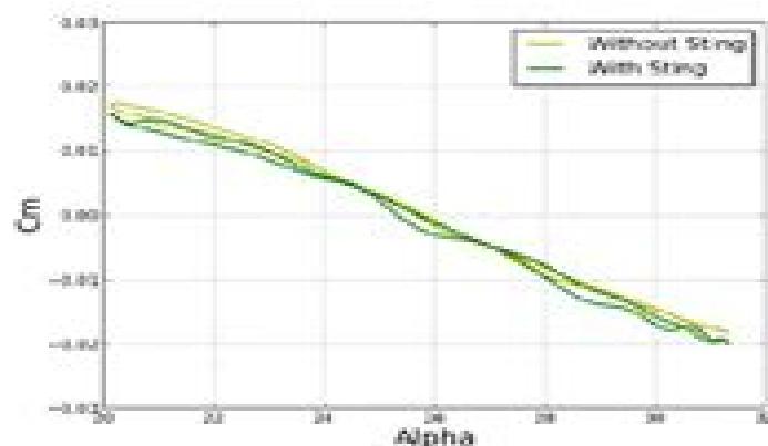
Figure 3 C_m history
