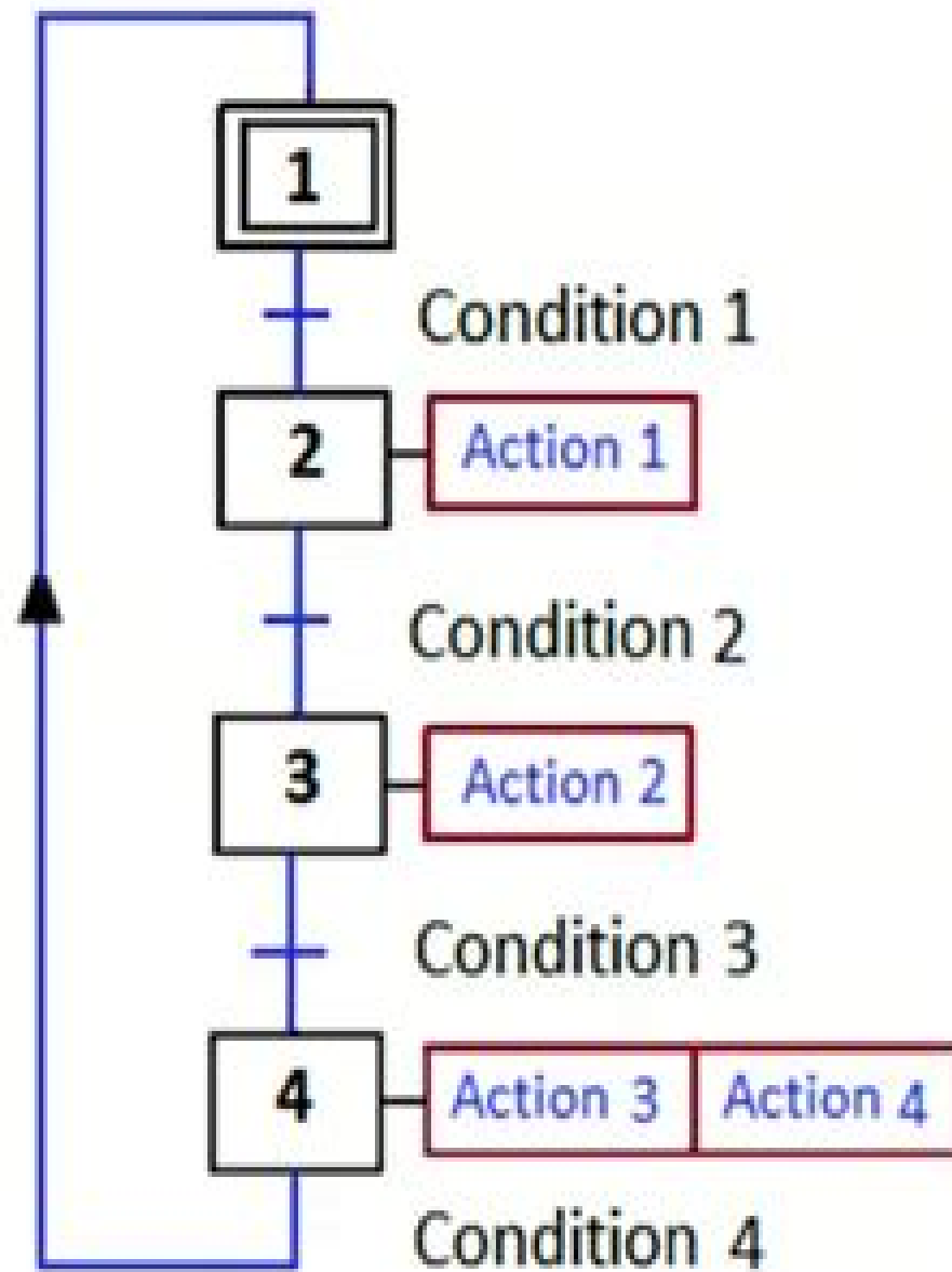
A Typical Sequential Function Chart
