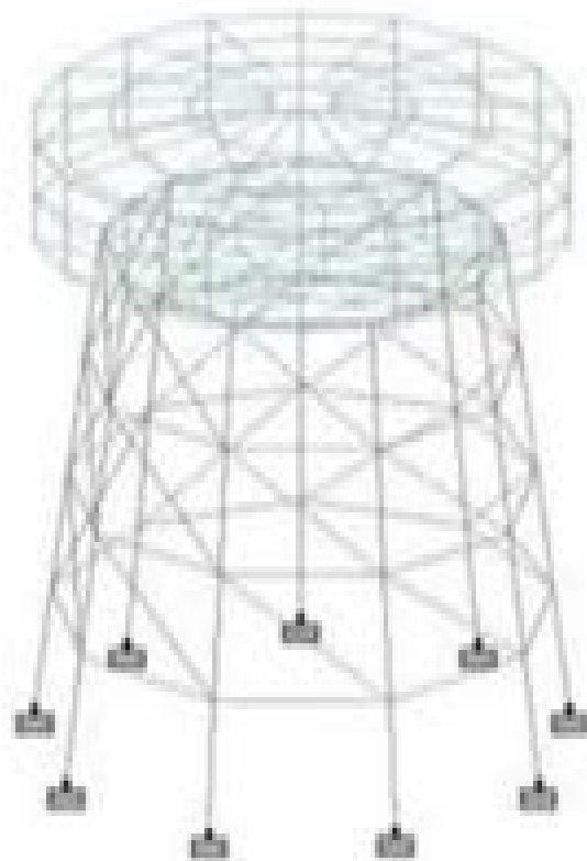
Fig.3 Model of Intze type water tank With Diagonal Bracing
