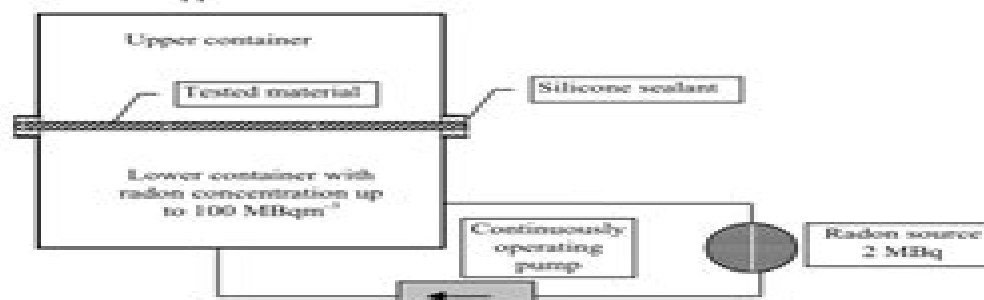
Fig. 1: Arrangement of the measuring appliance
