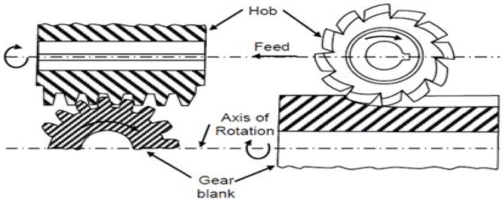
: Process of Gear Hobbing
