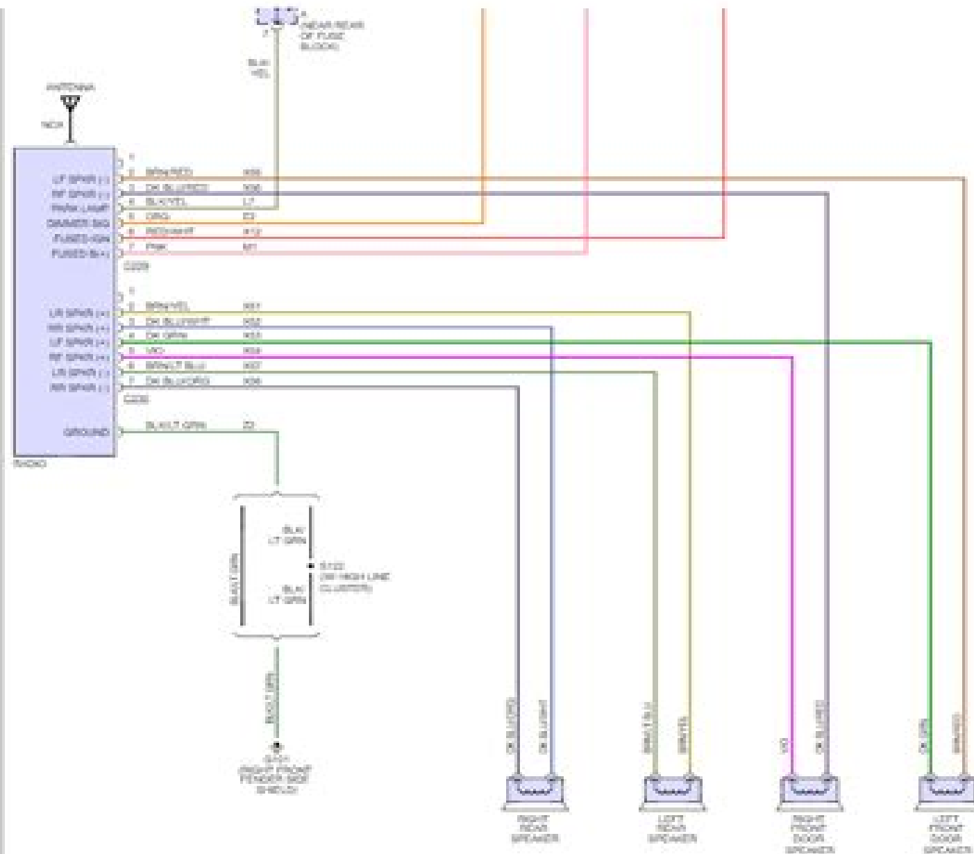
Fig 1: Radio Circuits, Base Radio
