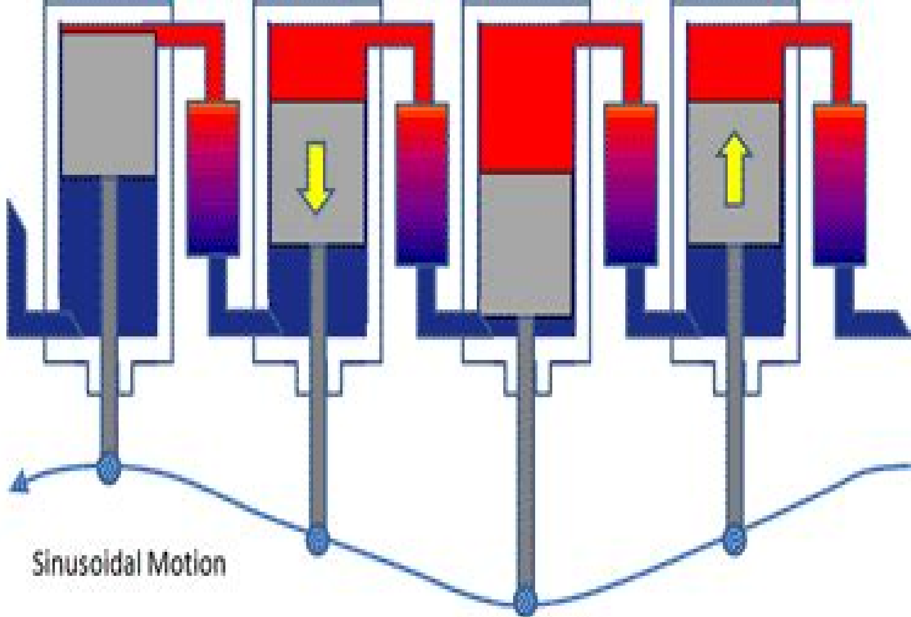
Double – Acting Stirling Engine
