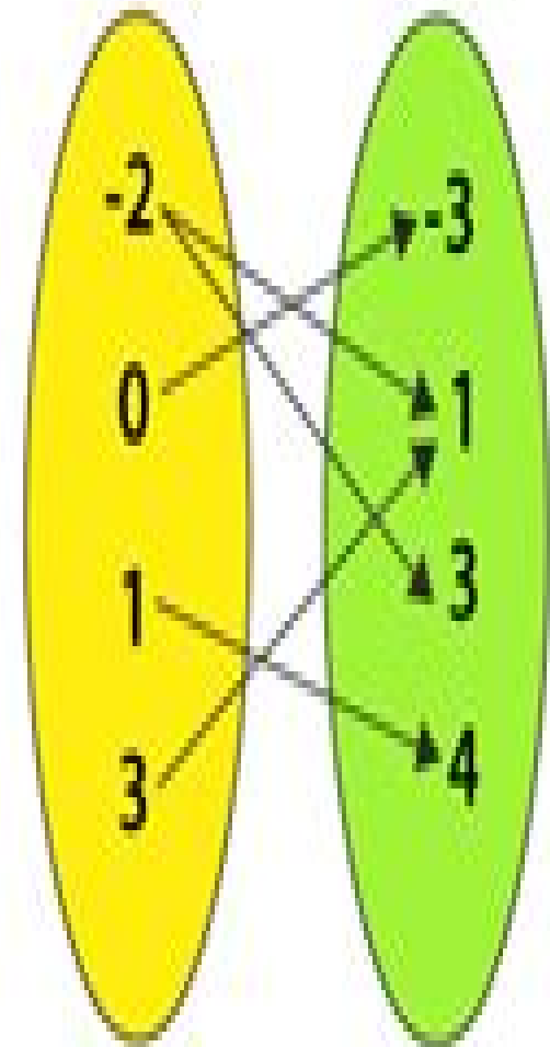
Relation in mapping diagram
