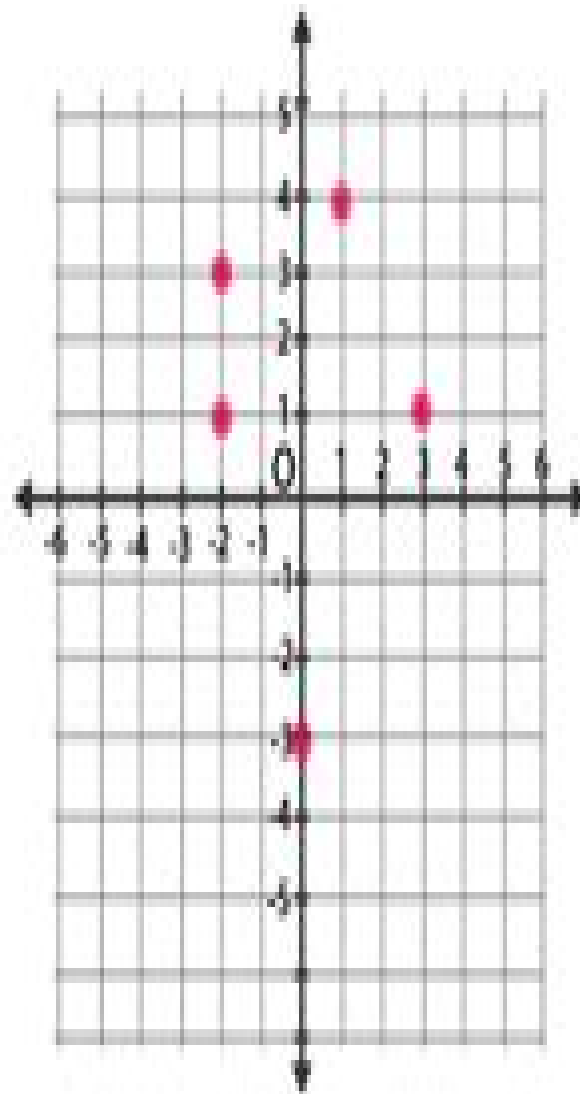
Relation in graph
