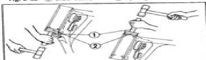
Fig. 2-63 ① driver handle (007749-6110000) ② Ball race driver attachment (007946-3290000)
