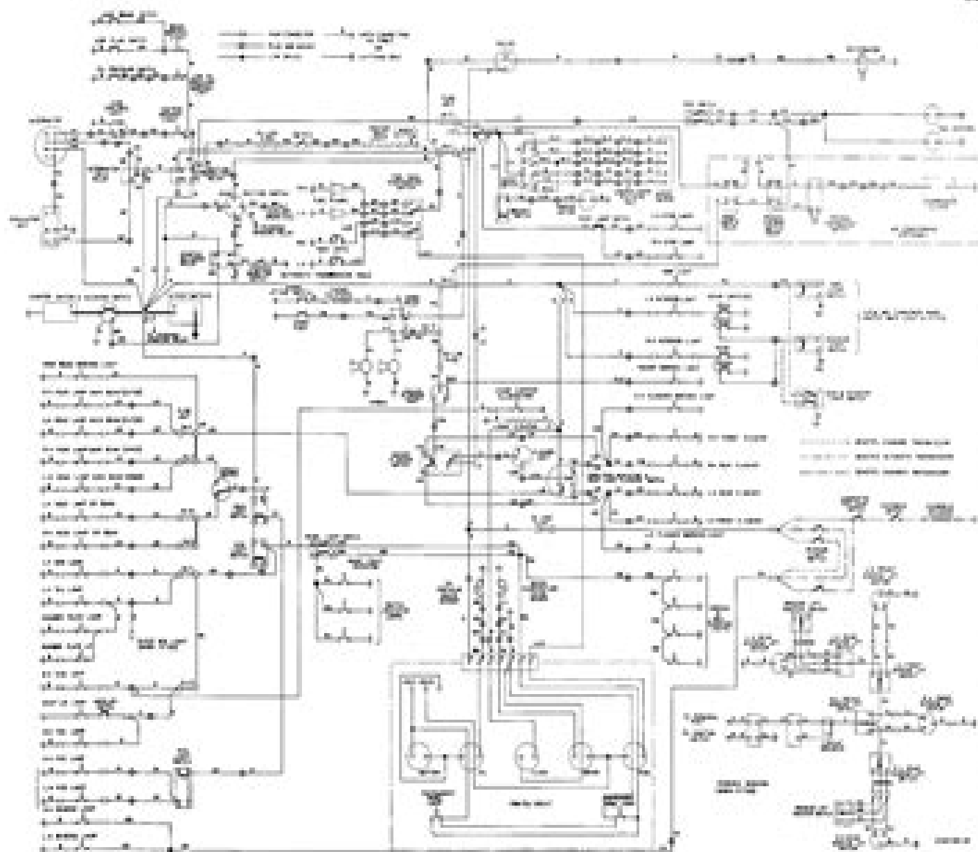
JAGUAR XJS WIRING DIAGRAM (W/SAFARI)
