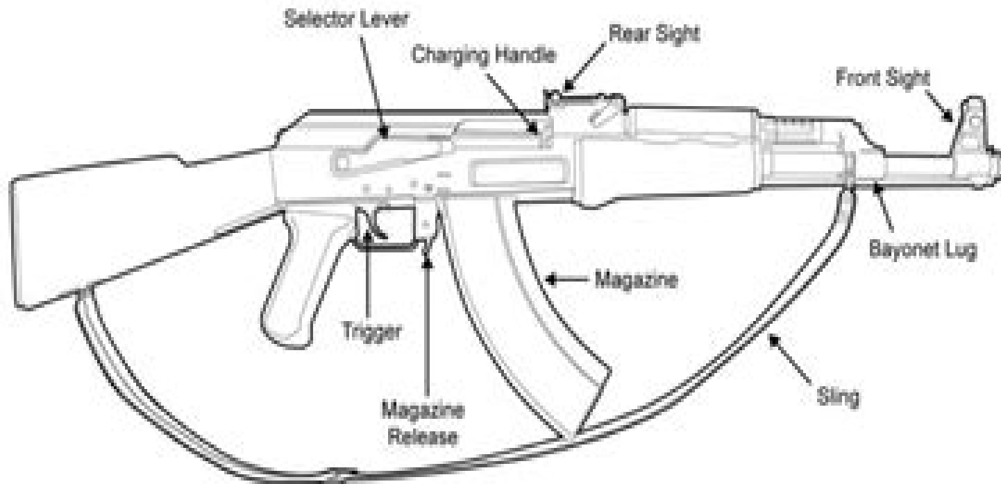
Figure 1. Right Side View of the Weapon.
