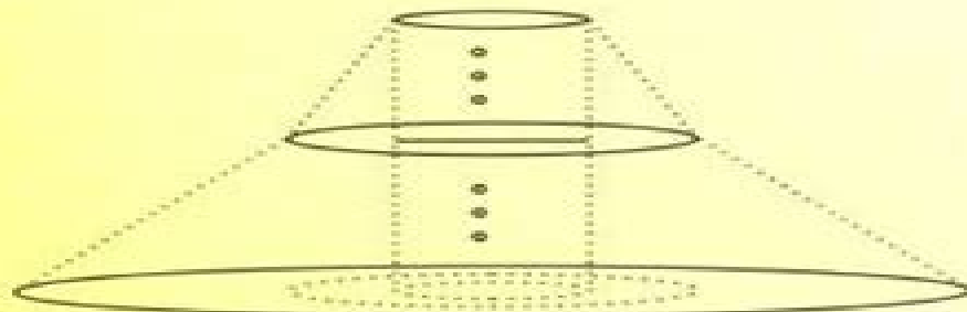
Abstraction hierarchy
