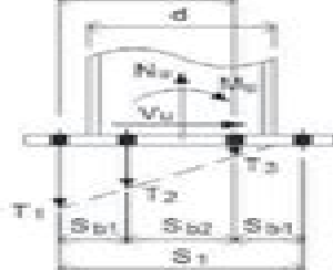
4 BOLT LINE
