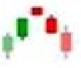
evening star
