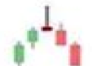
shooting star
