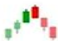
dark cloud
