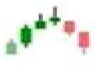
advance block
