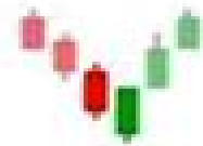
piercing line
