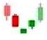
morning star
