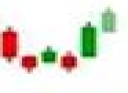
tower bottom
