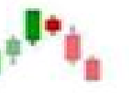
bearish harami
