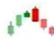
bearish engulfing
