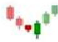
bullish engulfing
