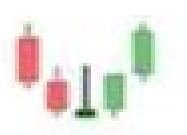
inverted hammer
