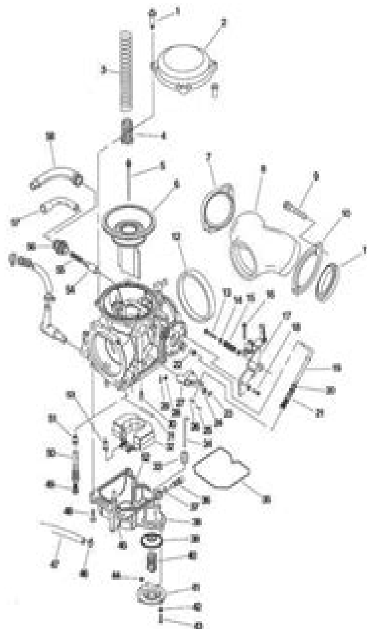
Figure 4-12. Carburetor
