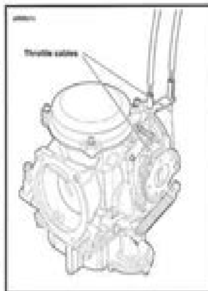
Figure 4-11. Throttle Cables
