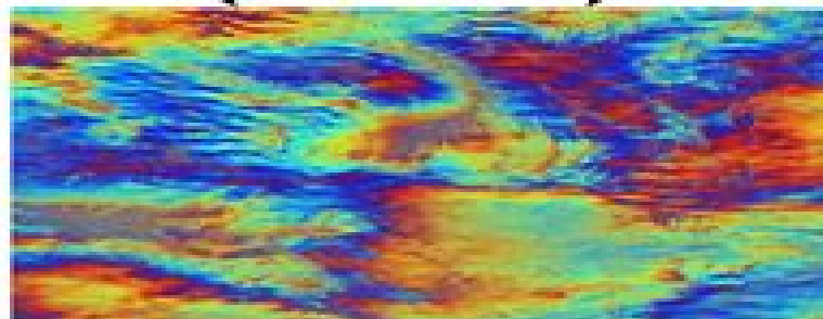
Final Interferogram
