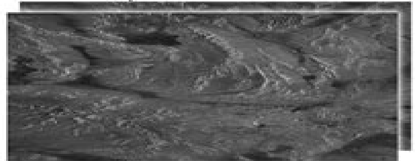
SLC Interferogram
