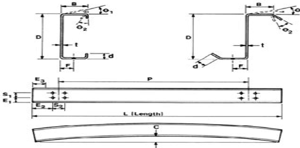
Figure 9.1: Cold-Formed Structural Members
