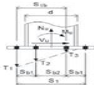
4 BOLT LINE
