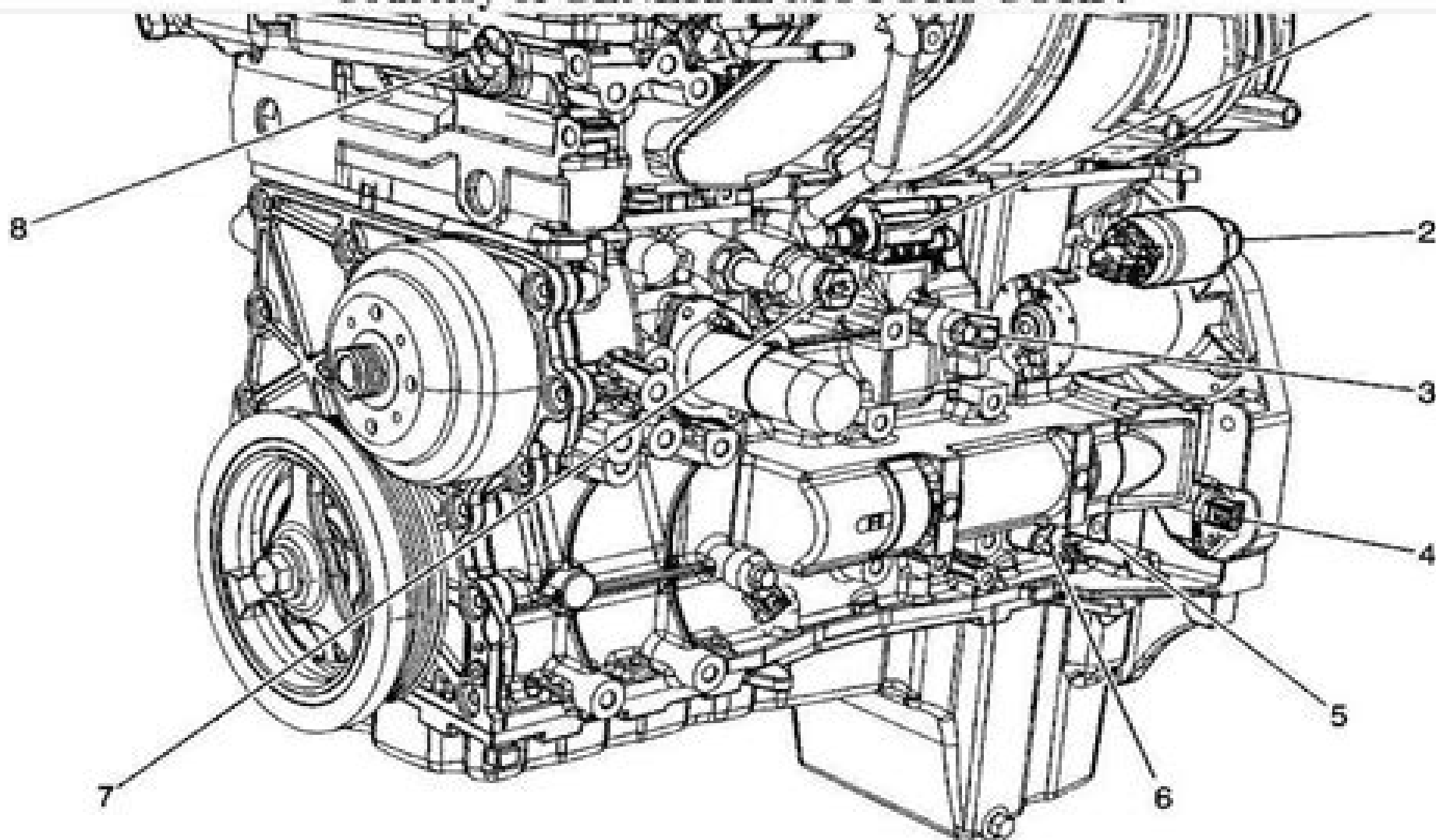
Fig. 19: Left Side Of Engine
