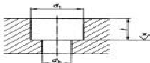
Figure 1. Counterbore
