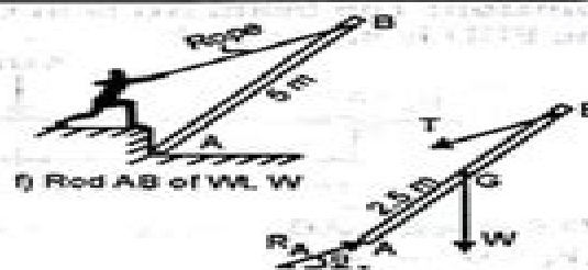
FBD
