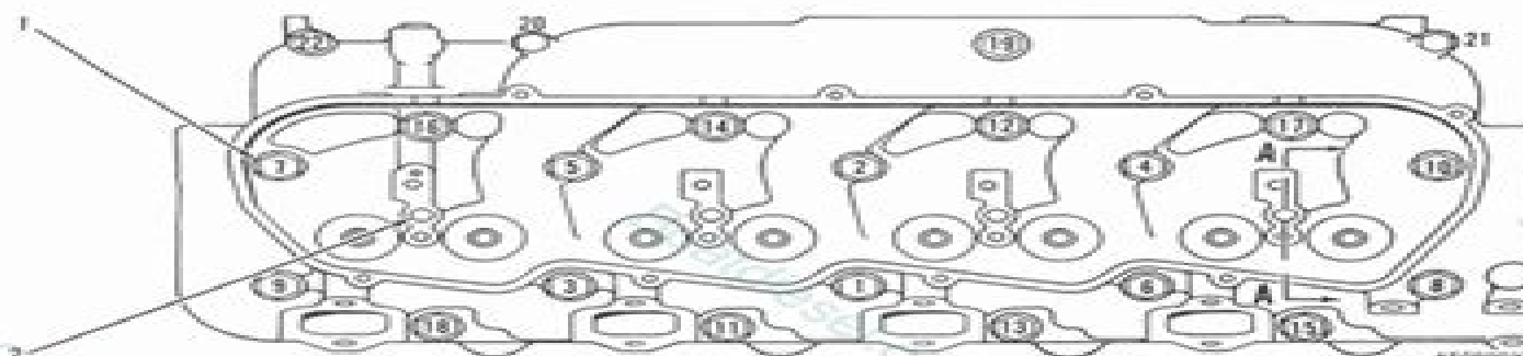
HEAD BOLT LOCATION AND TIGHTENING SEQUENCE
