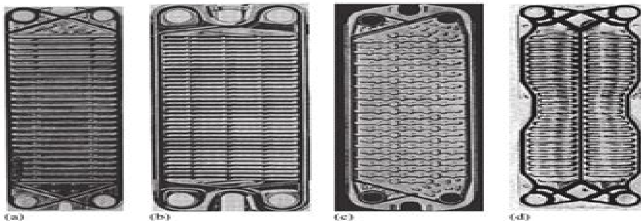
Figure 2.6: Plates with different surface corrugation patterns produced during the 1940s by different manufacturers: (a) APV HM, (b) Alfa Laval P12, (c) Schindt Sigma 20, and (d) Ahlborn.
