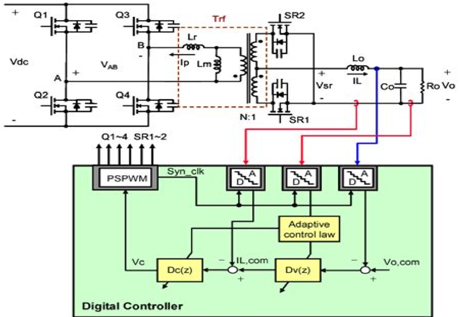
Fig. 1. Overall system block diagram of the digital current-mode control for the FB-PS DC-DC converter.
