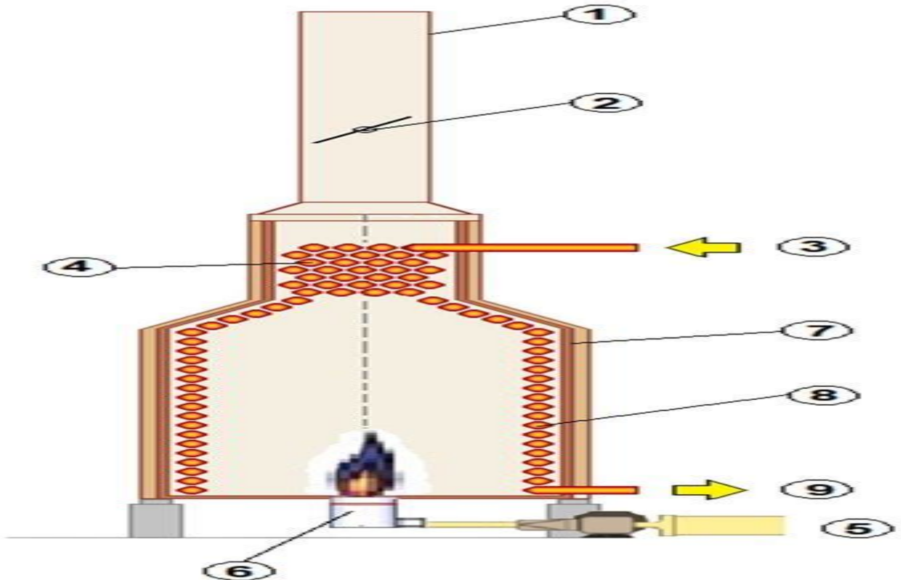
Fig 1. Direct Fired Heater 1 Chimney 2 Damper 3 Product inlet 4 Convection zone 5 Combustion air inlet 6 Burner 7 Refractory 8 Radiation zone 9 Product outlet
