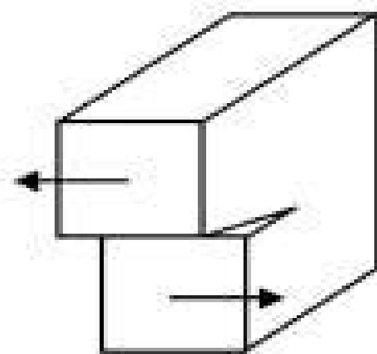
Mode 3 (Tearing)
